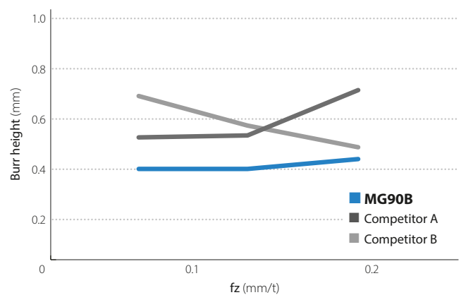
Burr height
