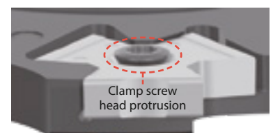
Clamp screw condition when using incompatible inserts and clamp screws
